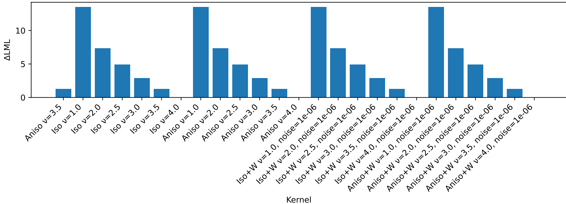
Difference from best LML (T8)
